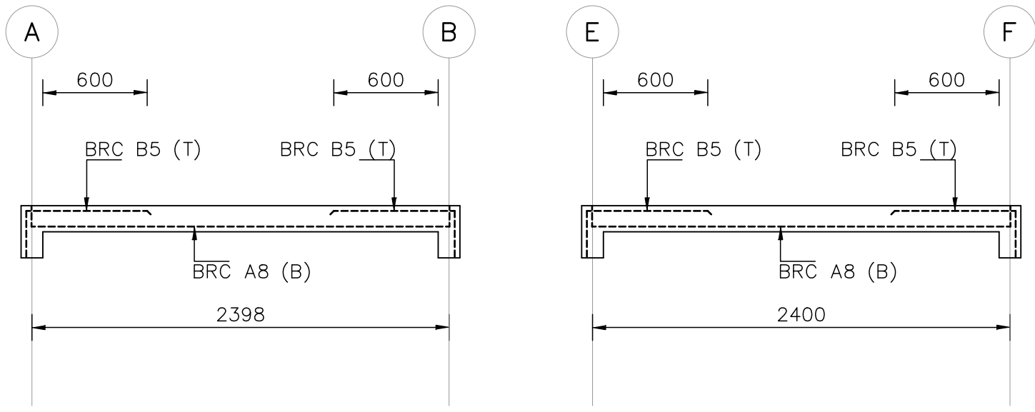
FS1 (150 thk.) Slab Cut Section No. 1 FS4 (150 thk.)
