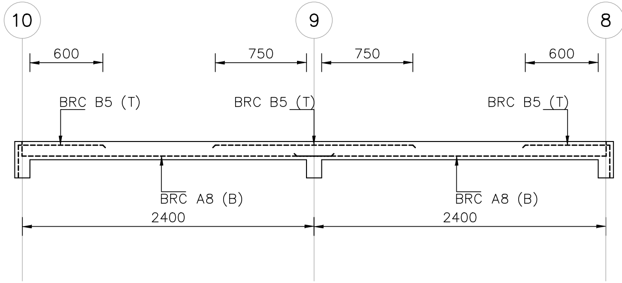
FS4 (150 thk.) FS3 (150 thk.) Slab Cut Section No. 2
